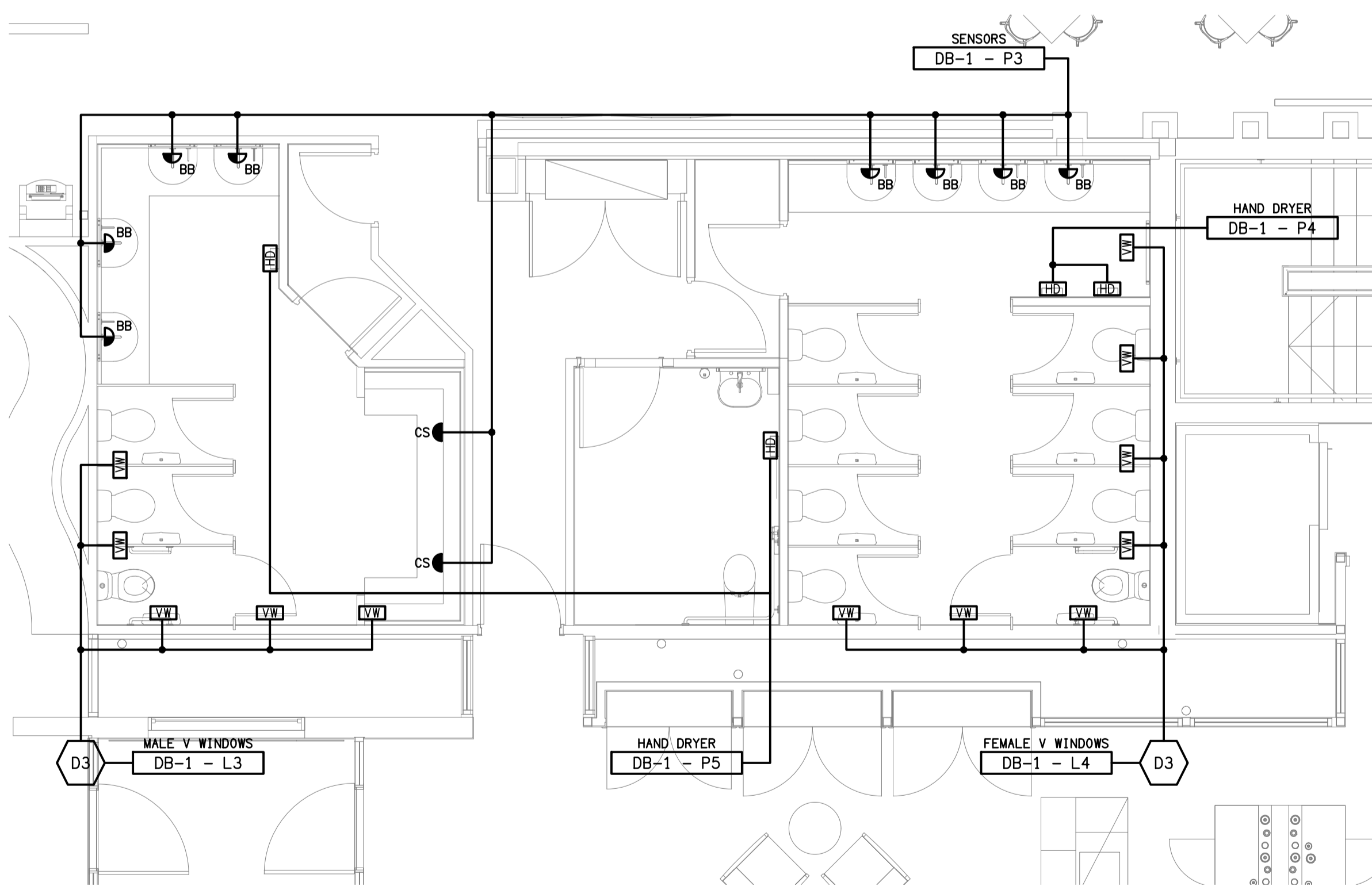
ZONE 3 RESTAURANT AMENITIES FLOOR PLAN SCALE 1: 50
