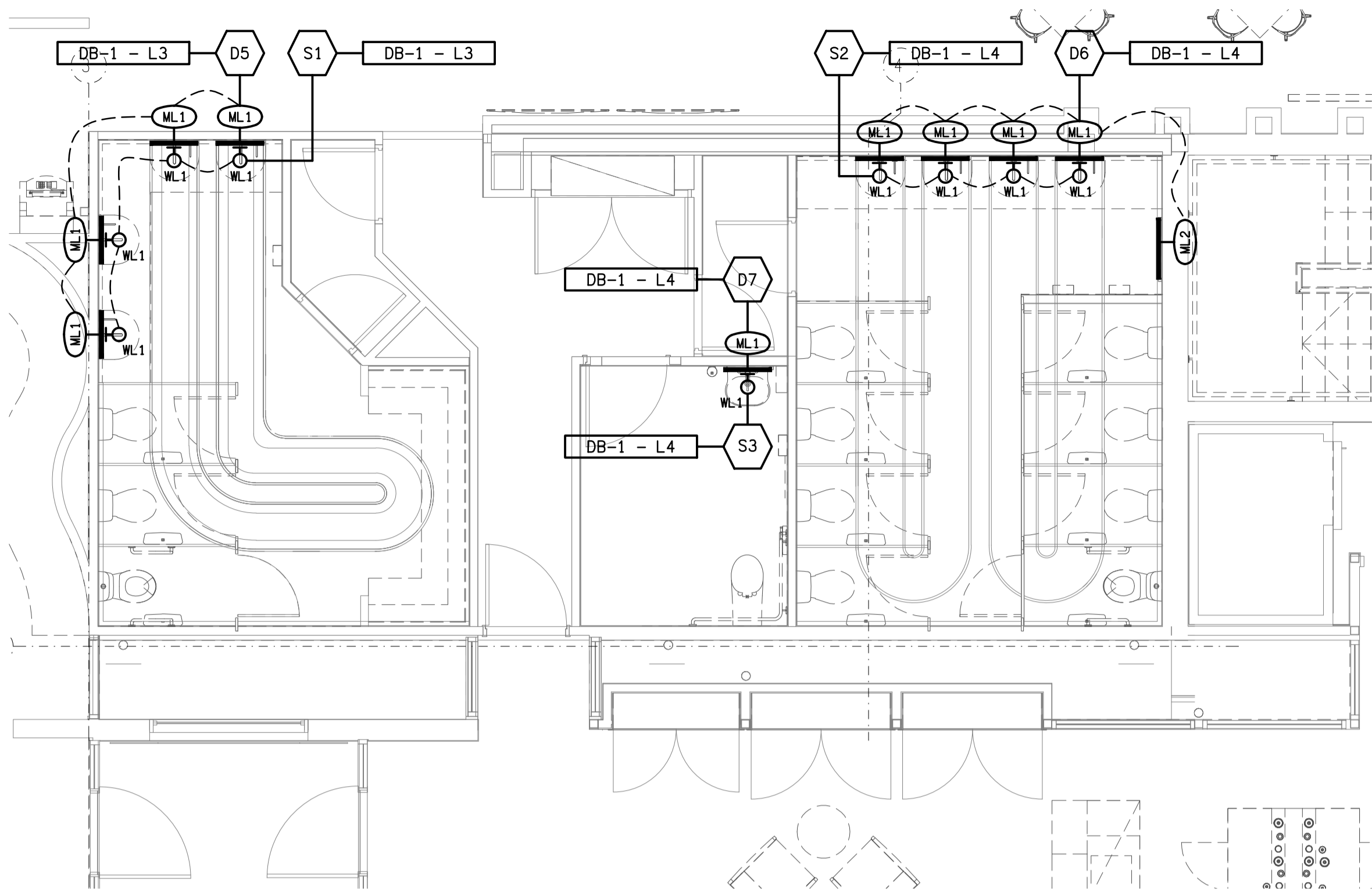
ZONE 3 RESTAURANT AMENITIES WALL MOUNTED LIGHTING SCALE 1: 50
