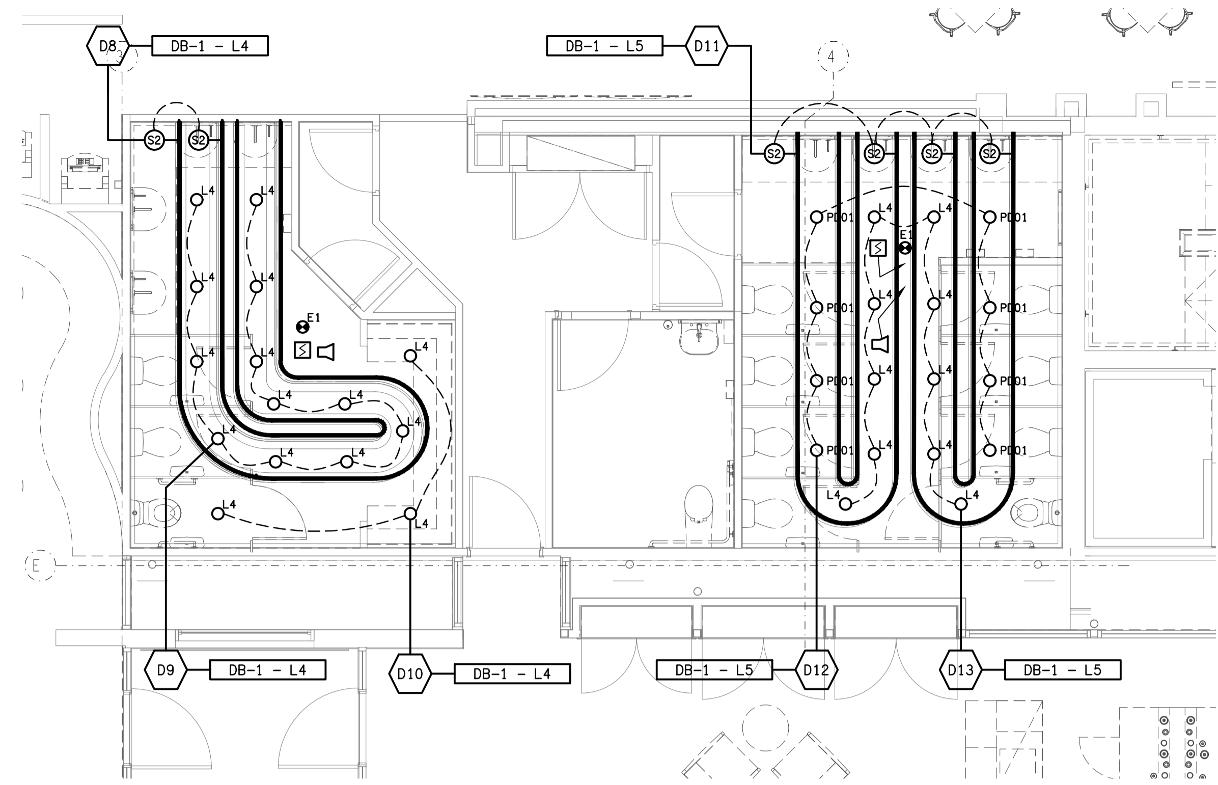
ZONE 3 RESTAURANT AMENITIES REFLECTED CEILING PLAN SCALE 1: 50
