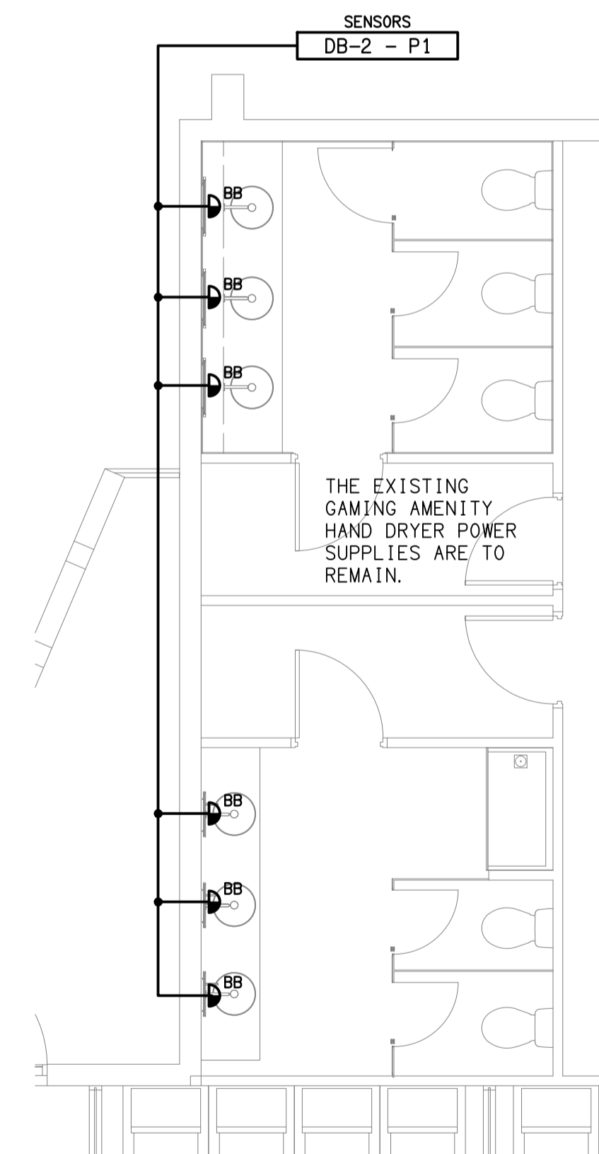
ZONE 4 GAMING AMENITIES FLOOR PLAN SCALE 1: 50
